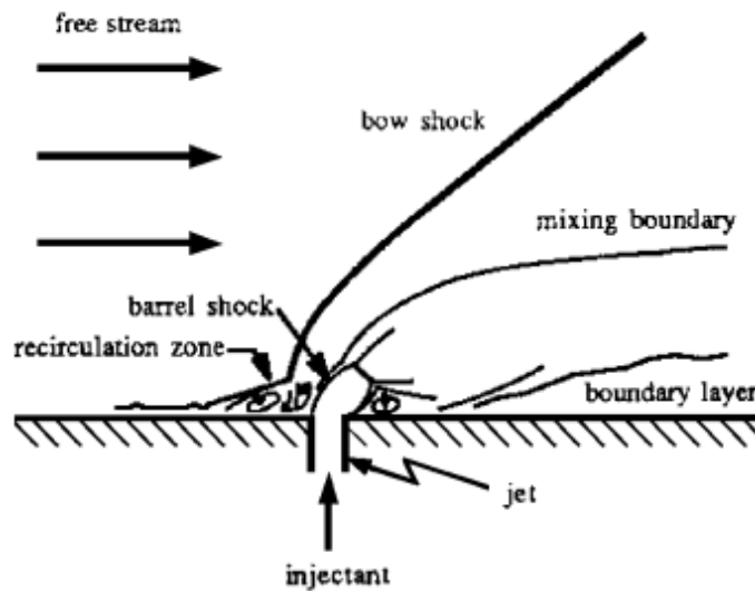
Figure 10: Normal fuel injection.
