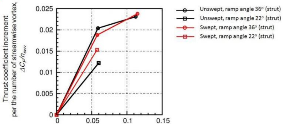
Figure 7: Comparison between the thrust coefficient increment of swept and unswept ramp.
